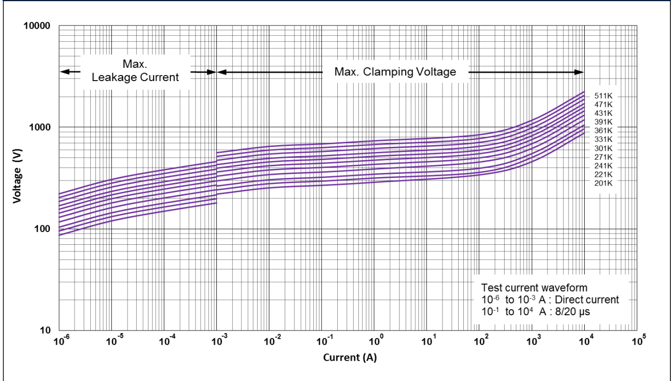
CNR-20V201K to CNR-20V511K V-I Curves
