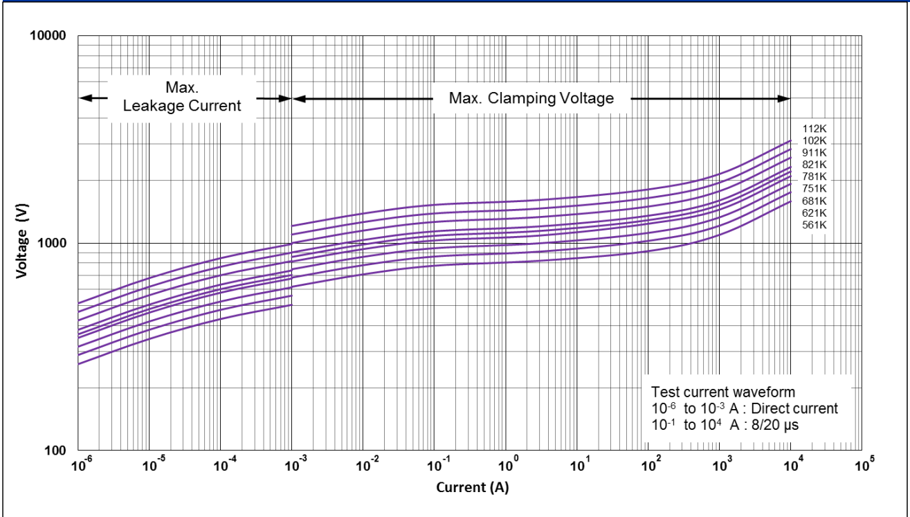
CNR-20V561K to CNR-20V112K V-I Curves
