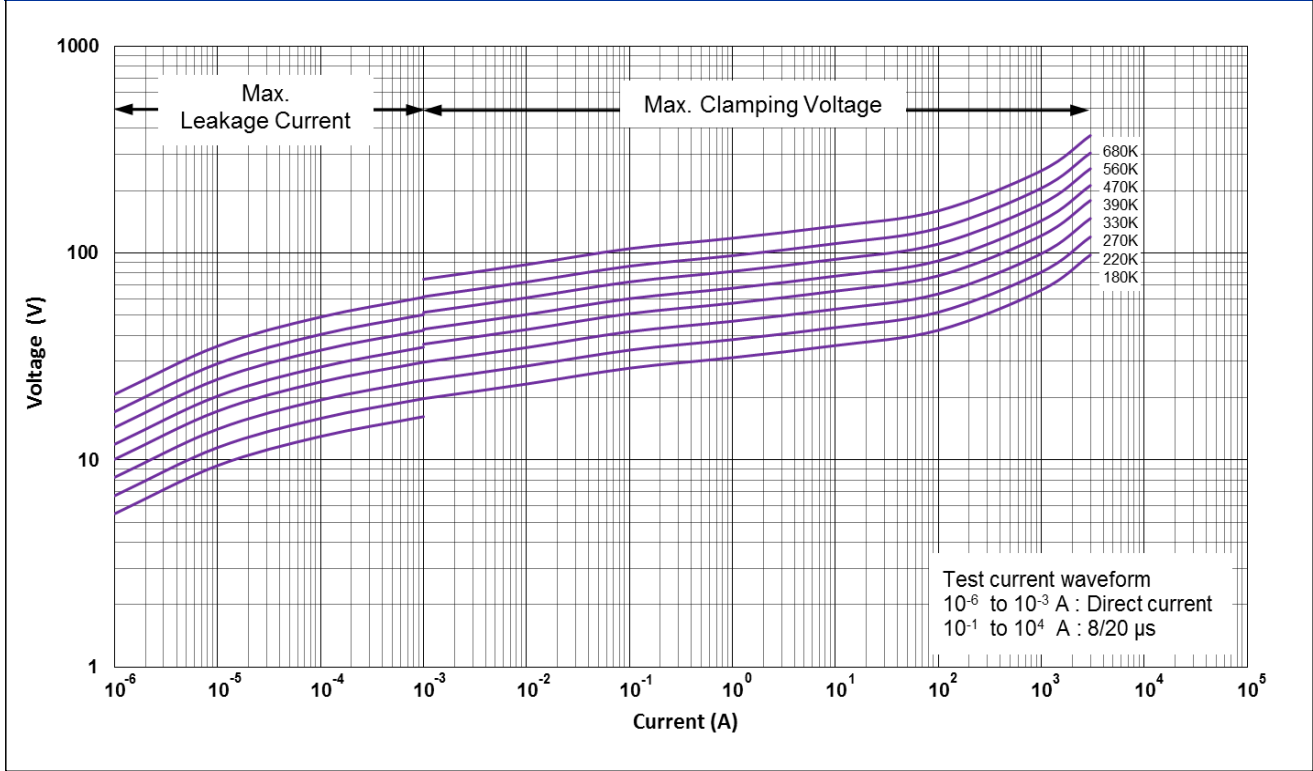
CNR-14N180K to CNR-14N680K V-I Curves
