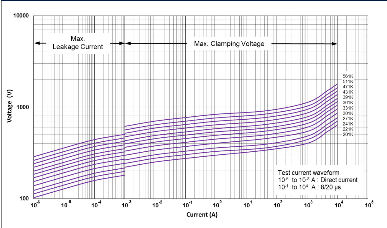
CNR-14N201K to CNR-14N561K V-I Curves
