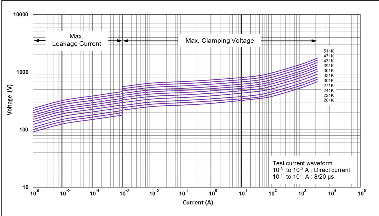
CNR-10V201K to CNR-10V511K V-I Curves
