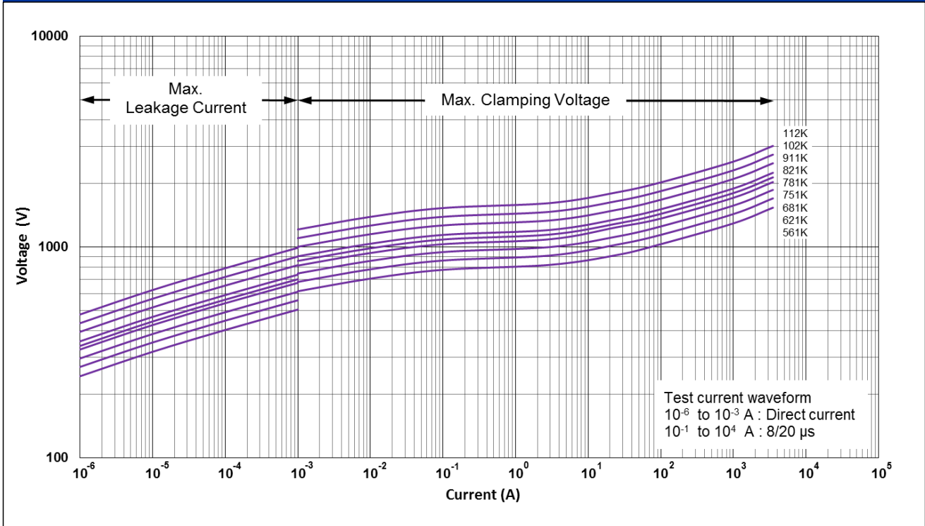
CNR-10V561K to CNR-10V112K V-I Curves
