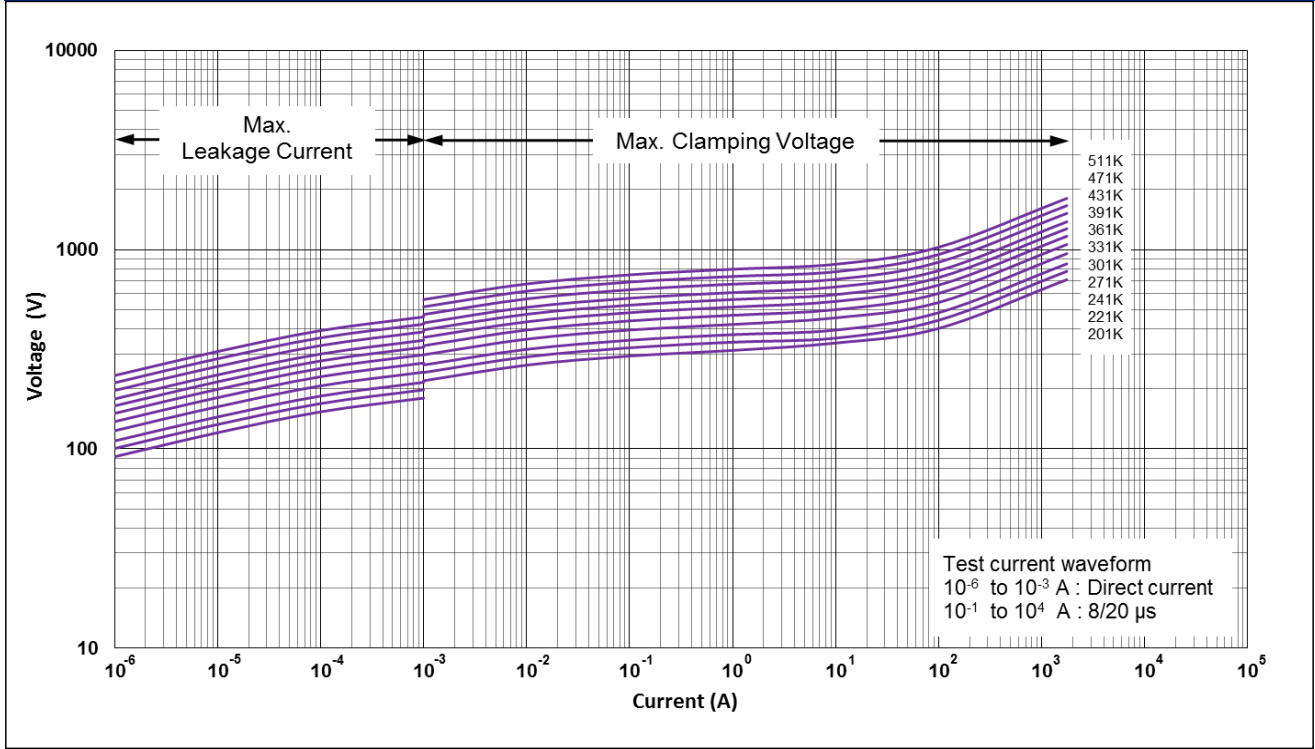
CNR-07V201K to CNR-07V511K V-I Curves
