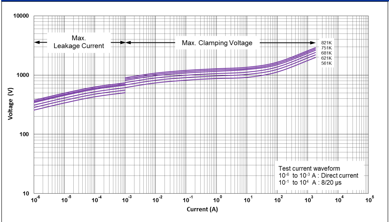
CNR-07V561K to CNR-07V821K V-I Curves
