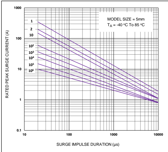
CNR-05N180K to CNR-05N680K
