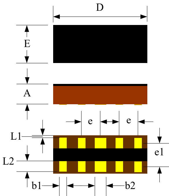
Package outline
