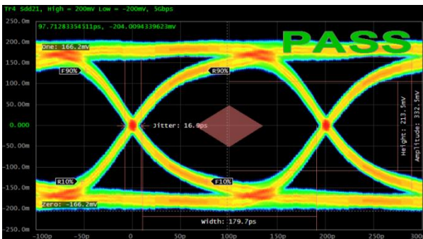
USB3.0 Mask at 5.0 Gb/s without UESD
