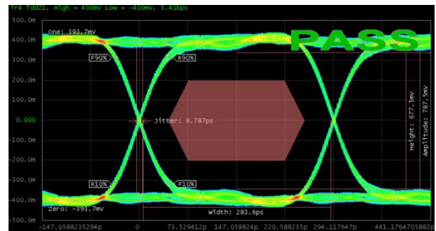
HDMI1.4 Mask at 3.4 Gb/s with UESD
