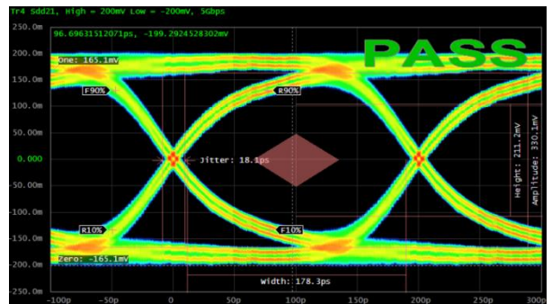
USB3.0 Mask at 5.0 Gb/s with UESD
