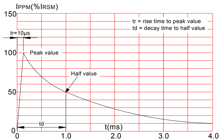
FIG.2: Pulse waveform
