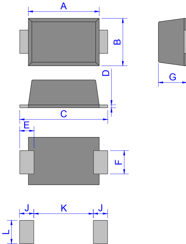
SOD-123FL
