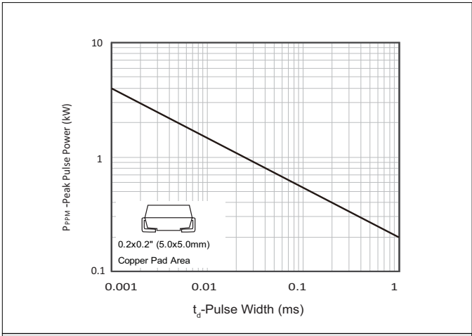
Figure 2 - Peak Pulse Power Rang Curve
