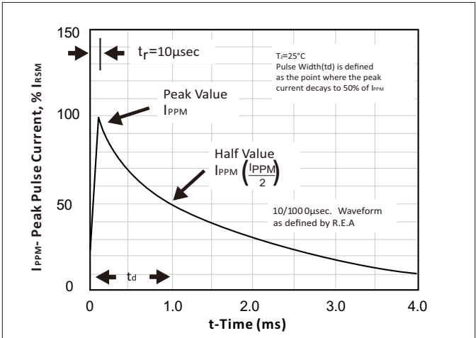
Figure 4 - Pulse Waveform - 10/1000µS
