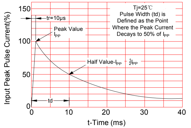
FIG.2: Pulse Waveform
